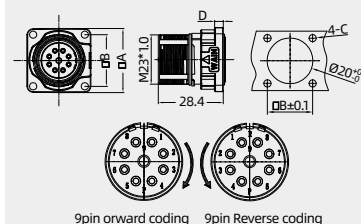
9pin orward coding 9pin Reverse coding
